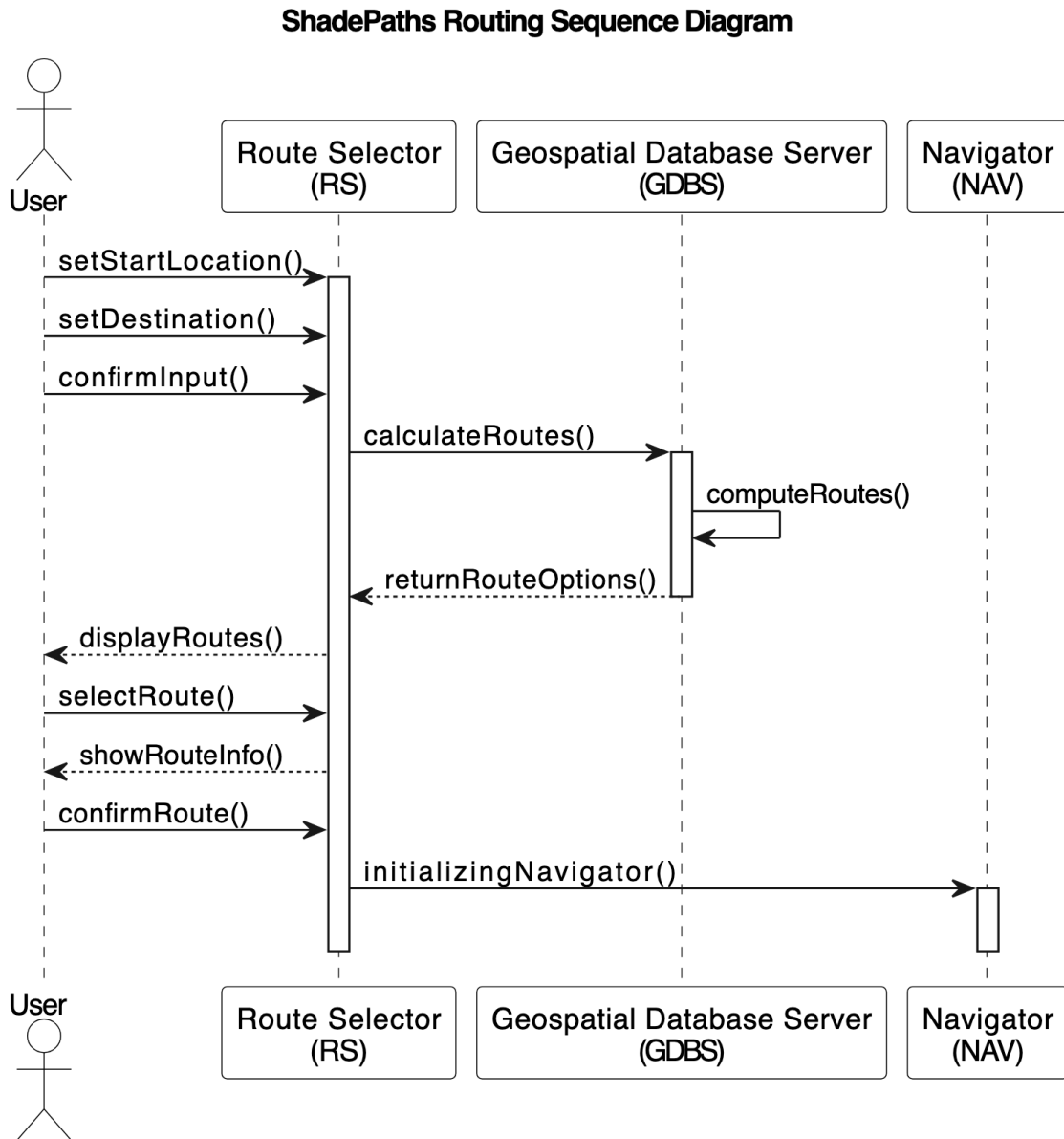
Figure 5: Sequence Diagram
