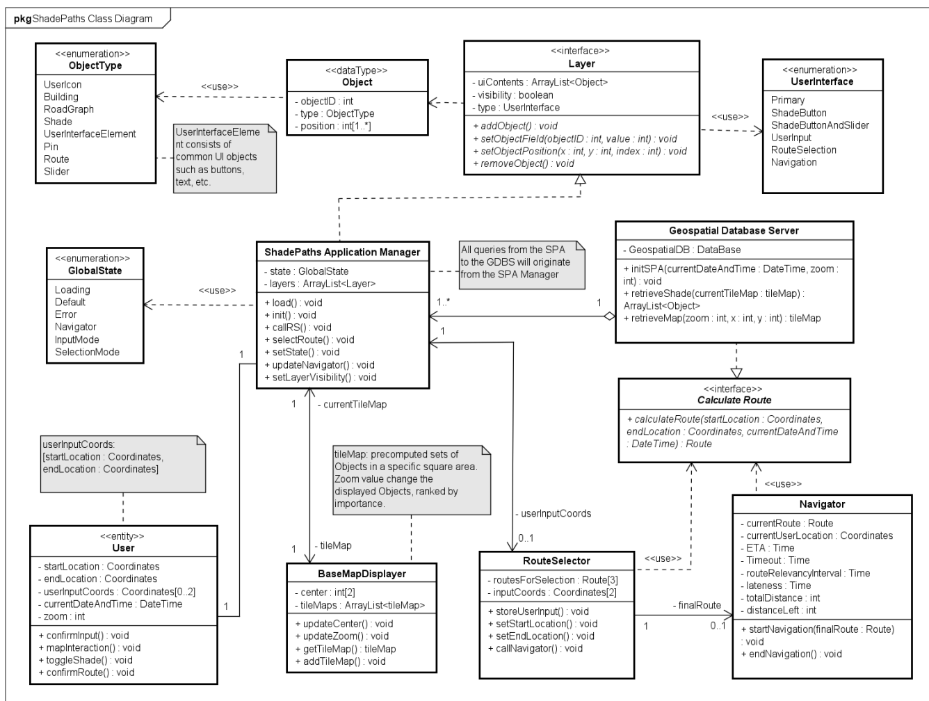
Figure 1: Class Diagram
