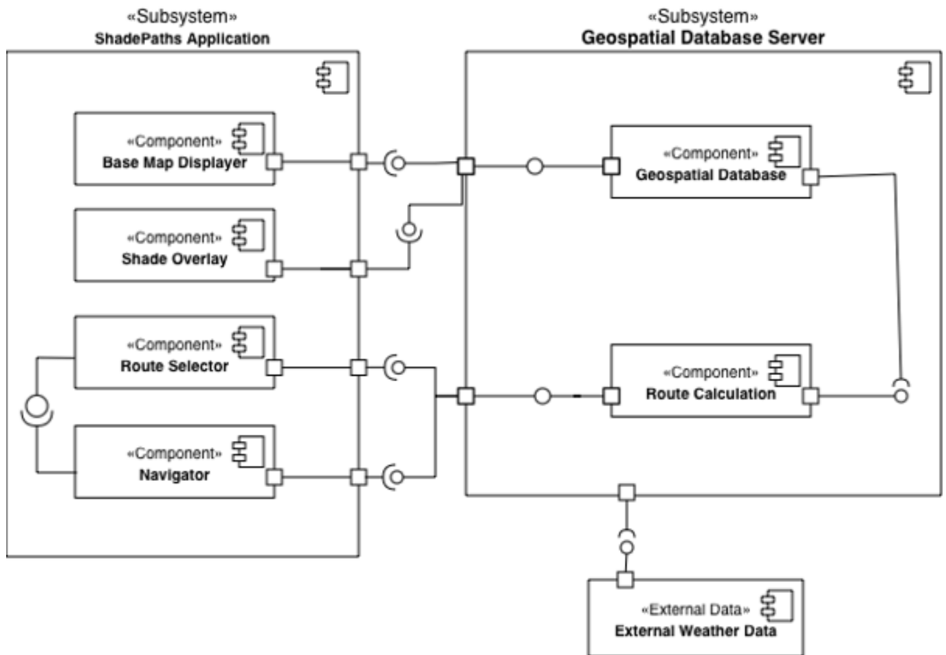
Figure 3: Component Diagram
